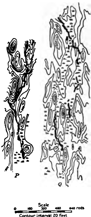
FIG. 342. — Small sketch maps showing the relationships in size, proportions, and orientation of drumlins and eskers in southern Wisconsin. The eskers are in solid black (after Alden).
